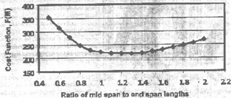
FIG 2 - APPROXIMATE OPTIMISATION CURVE FOR 3- SPAN BRIDGE
